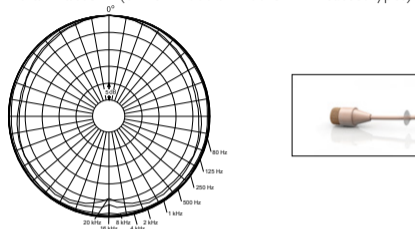
Polar Pattern (d:fine™ 4088 & 4088 Omni Headset types)
